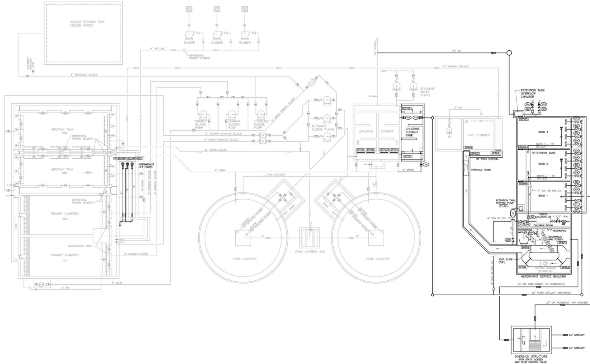
PROCESS FLOW SCHEMATIC NO SCALE
